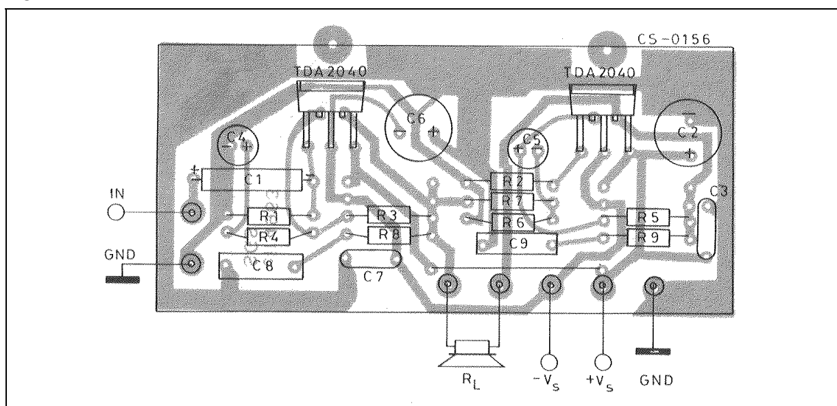
Figure 15 : P.C. Board and Components Layout for the Circuit of Figure 14 (1:1 scale)
